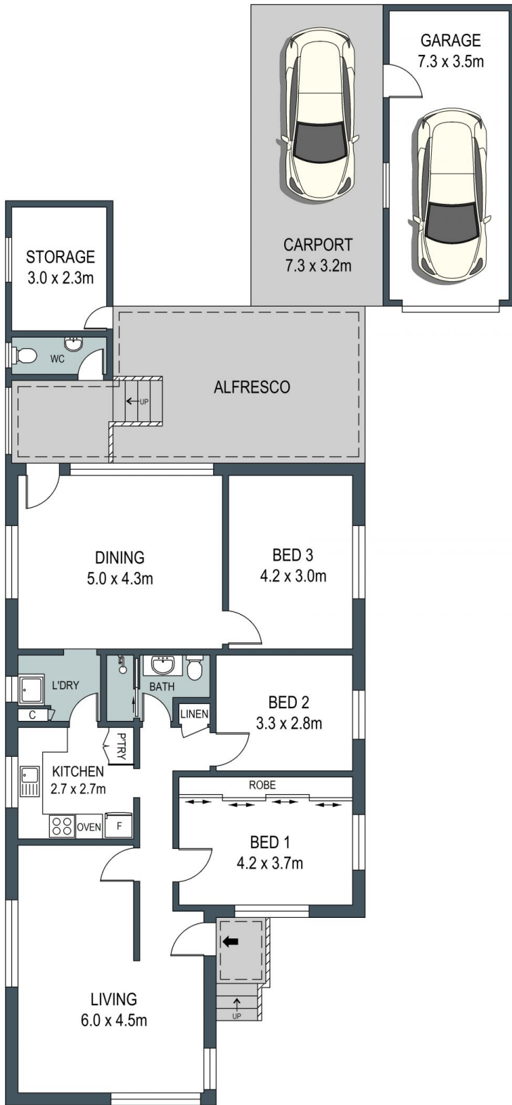
GROUND FLOOR
